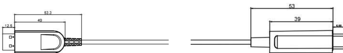
USB 3.1 Type A-C AOC Drawing
